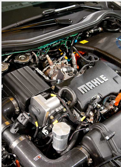
>> Range extender vehicle installation
